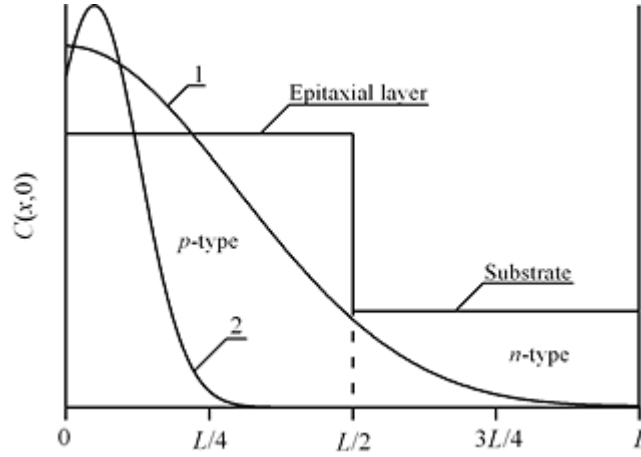
Fig. 1. Initial distributions of dopants and types of conductivity in the considered two-layer structure.
