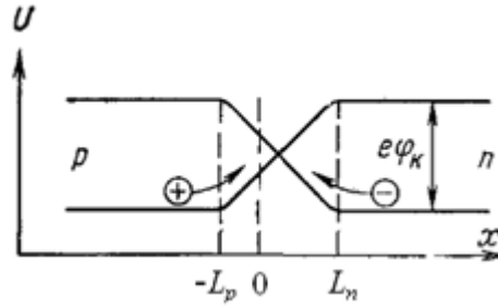
Fig. 2. Qualitative structure of p-n-junction.
