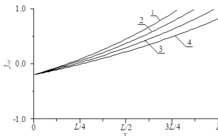
Fig. 4. Typical distributions of the diffusion component of current of charge carriers at different values of dose of radiation processing in implanted-junction rectifier.
