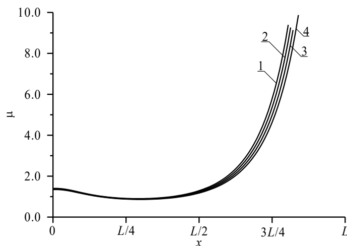
Fig. 3. Typical distributions of charge carrier mobility at different values of dose of radiation processing in implanted-junction rectifier.
