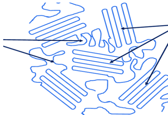
Fig. 6. Amorphous and crystalline regions of a polymer (plastics) [92].
